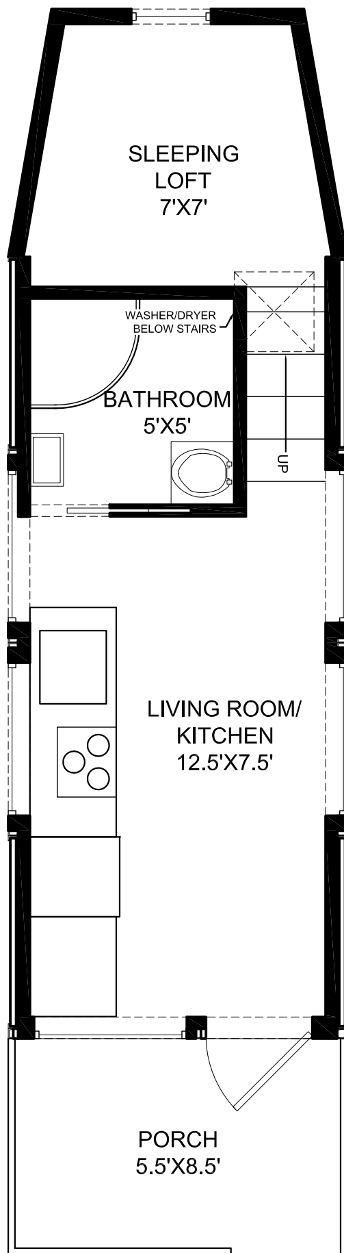
FLOOR PLAN NOT TO SCALE
